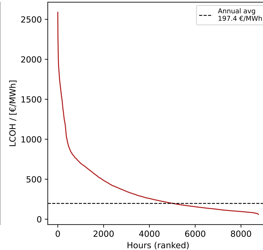
LCOH Duration Curve
