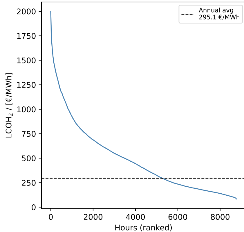
LCOH 2 Duration Curve
