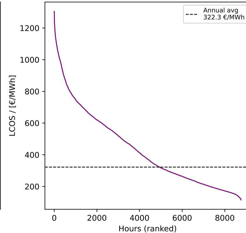
LCOS Duration Curve
