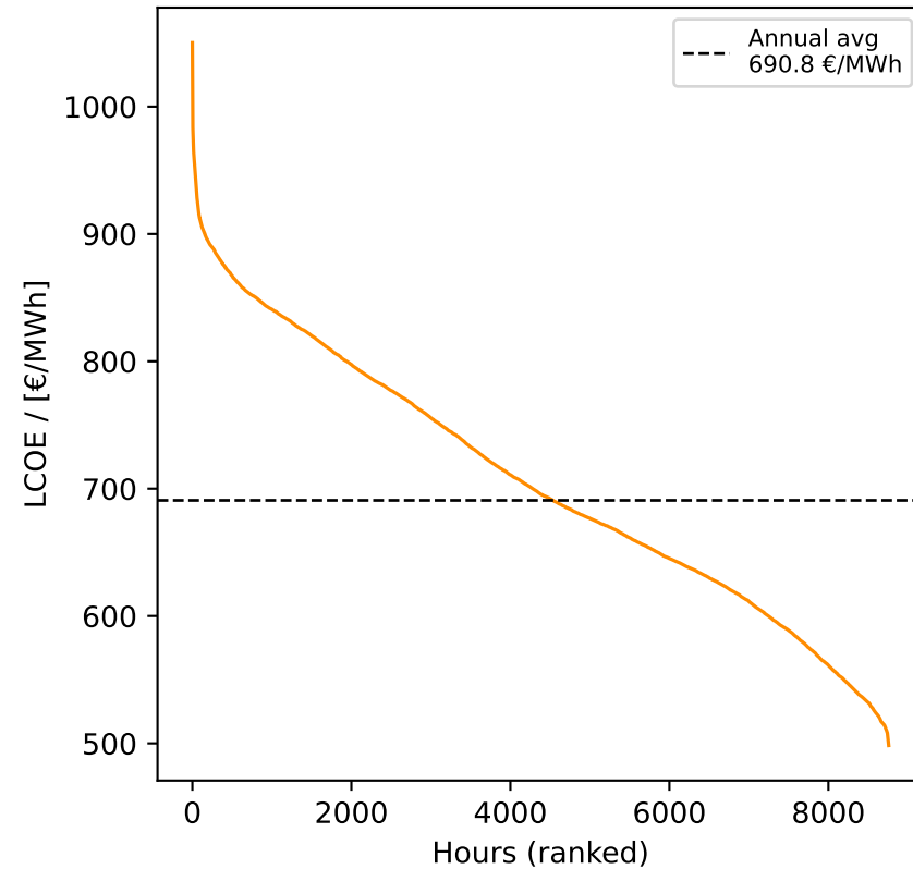
LCOE Duration Curve
